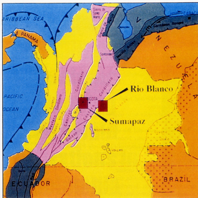
A geologic map illustrating the major tectonics of Colombia. The areas of recent petroleum activity are along the flanks of the Eastern Cordillera. Sumapaz is located along the west flank, and Rio Blanco is on the east.
