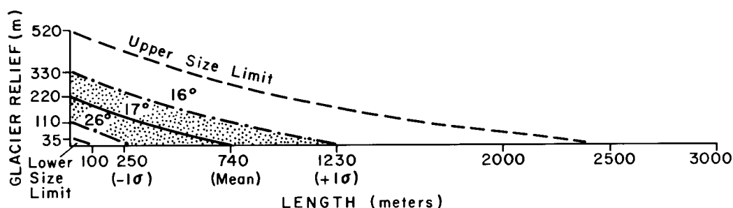
FIGURE 3. Generalized profile of 133 cirque glaciers in the field area showing mean altitude and length with 67% zone of occurrence ( \pm 1 standard deviation [ \sigma ]), upper and lower size limits, and slope of glacier surface. See also Table 1.
