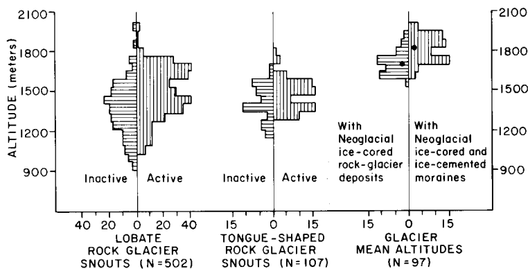
FIGURE 6. Summary of altitudinal distribution for glaciers and rock glaciers. Sixty-seven percent zone of occurrence for both active and inactive states shown. See also Table 3.
