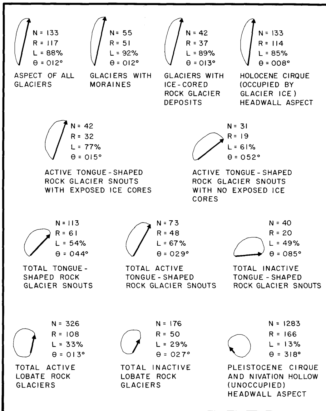
FIGURE 5. Graphical summary of aspect distribution data. See also Table 2. Note absolute scale varies so that strength of mean vectors (L) are of equal lengths if L = 100\% . L is shown by the thickened arrows, and equals R/N .
