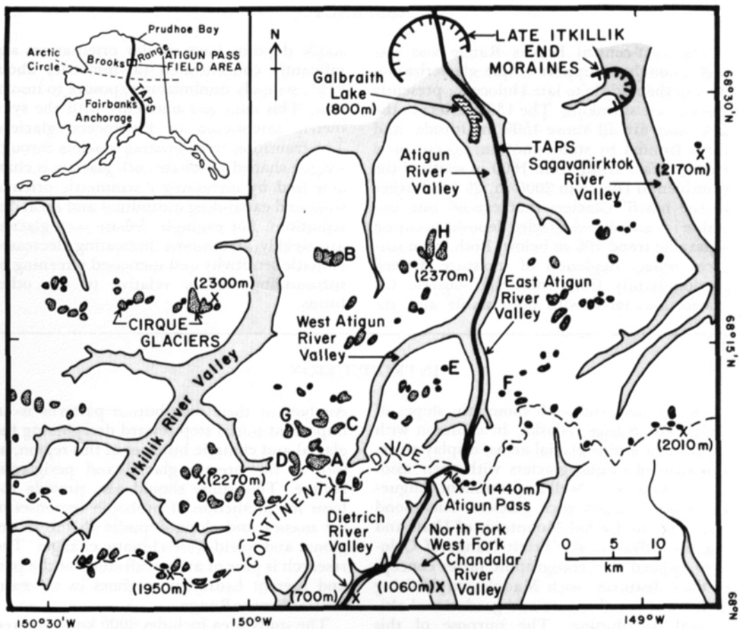
FIGURE 1. Atigun Pass field area showing present glaciers with major river valleys. Letters a-h refer to glaciers shown on Figure 4. Area west of Itkillik River studied with 1:63,360 USGS topographic sheets only for glacier aspect and mean elevation.
