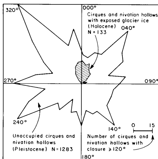
FIGURE 2. Orientation of cirques and nivation hollows in the field area. Basins with glacier ice are labeled as Holocene, those without ice are assumed to have been actively cut only during Pleistocene glaciations.
