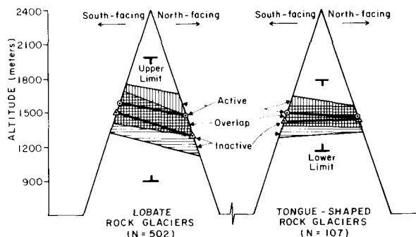
FIGURE 9. Comparison of altitudinal distribution of south-facing and north-facing rock glaciers. Those facing 090 and 270° were not included in analysis. The sixty-seven percent zone of occurrence about the mean is shown for both active and inactive states. See Table 3.
