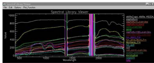
Field spectrometer measurements for different materials
